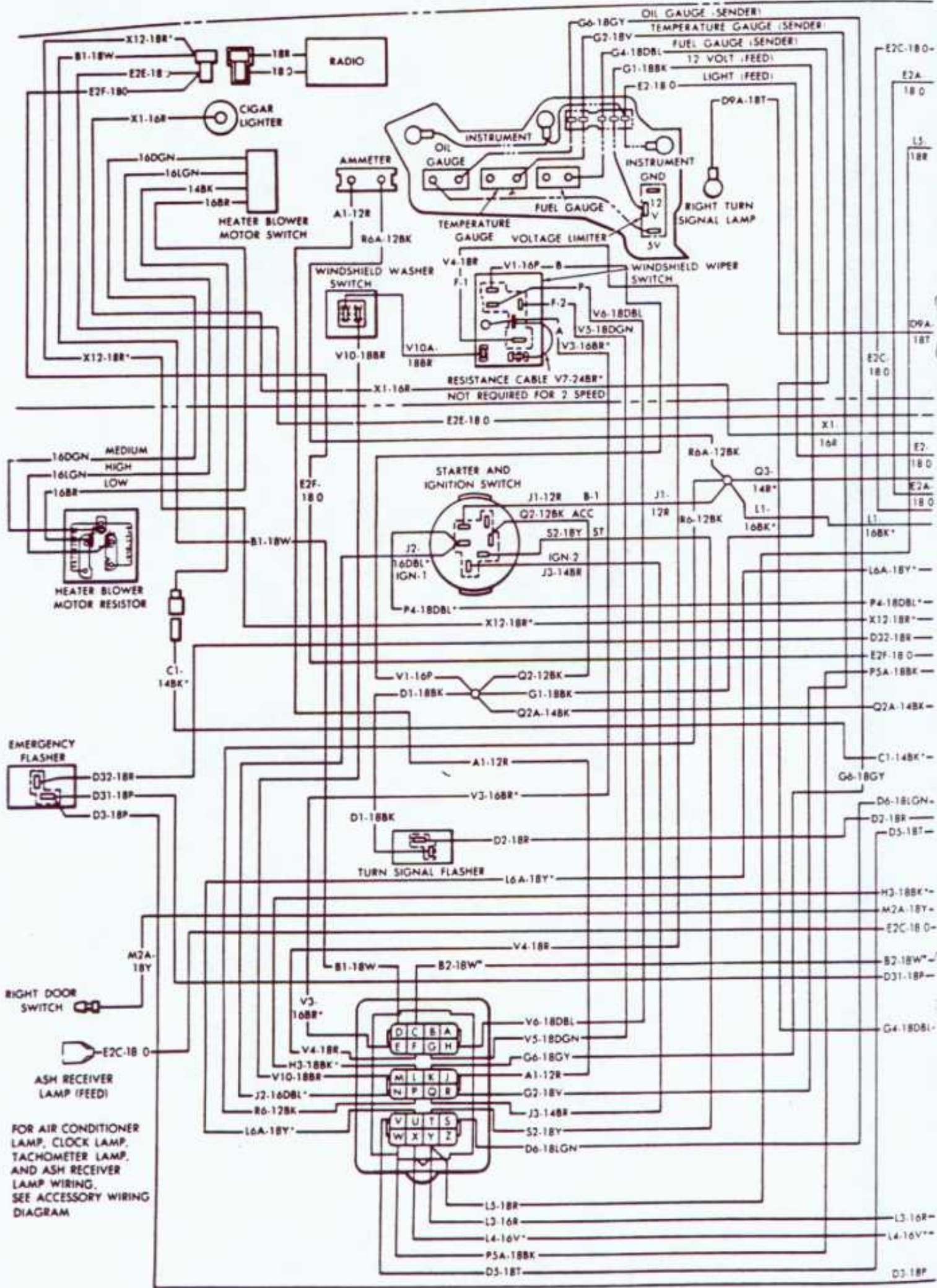
Instrument Panel
